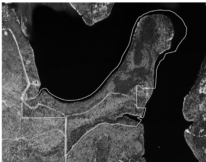
Fig. 2. Aerial photograph showing the boundary of the South Fork Native Plant Preserve Study Area. Note that boundary shown in lake represents low water level in October 2005.
